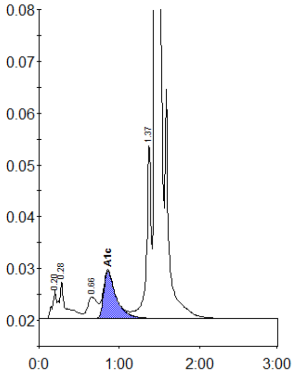
Peak table - ID: 10390862
